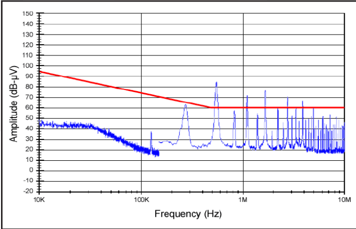
Figure 23: High frequency conducted emissions of standalone MQFL-28-05S, 5vout module at 120W output, as measured with Method CE102. Limit line is the 'Basic Curve' for all applications with a 28V source.
