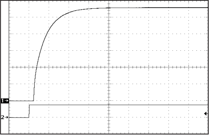
Turn-on transient at full resistive load and zero output capacitance initiated by ENA1. Input voltage pre-applied. Ch 1: Vout (5V/div). Ch 2: ENA1 (5V/div).
