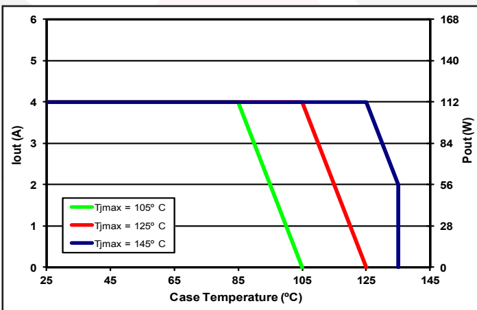
Output Current / Output Power derating curve as a function of T_{case} and the Maximum desired power MOSFET junction temperature at V_{in} = 28V (see Note 14).
