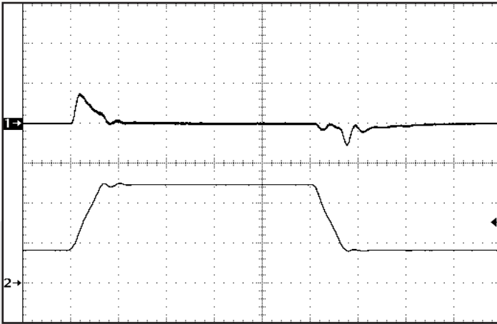
Figure 13: Output voltage response to step-change in input voltage (16V-50V-16V). Load cap: 10 \mu F, 100 m \Omega ESR tantalum cap and 1 \mu F ceramic cap. Ch 1: Vout (500mV/div). Ch 2: Vin (20V/div).
