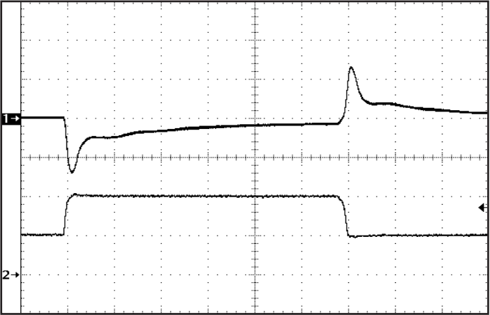
Figure 11: Output voltage response to step-change in load current (50%-100%-50% of Iout(max)). Load cap: 1μF ceramic cap and 10μF, 100 mΩ ESR tantalum cap. Ch 1: Vout (500mV). Ch 2: Iout (2A/div).
